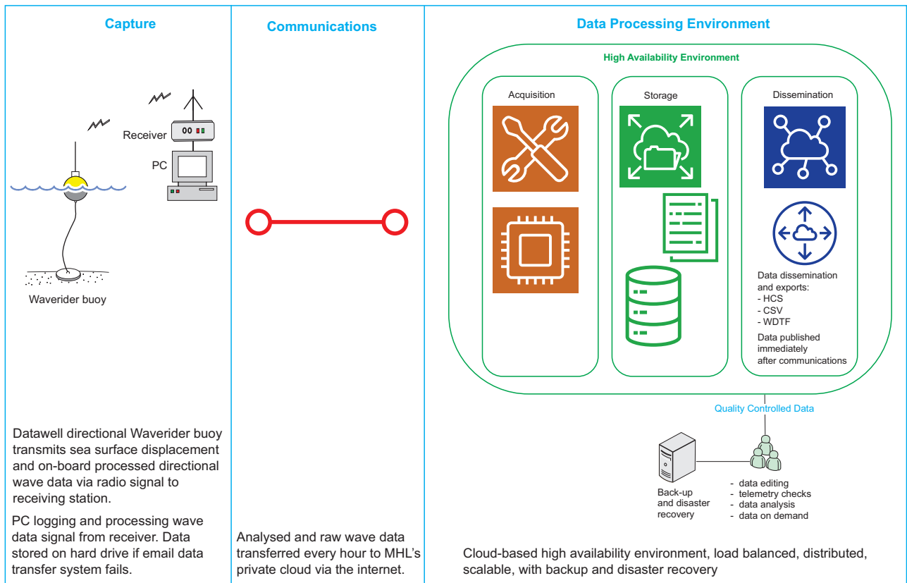
Data transfer schematic
